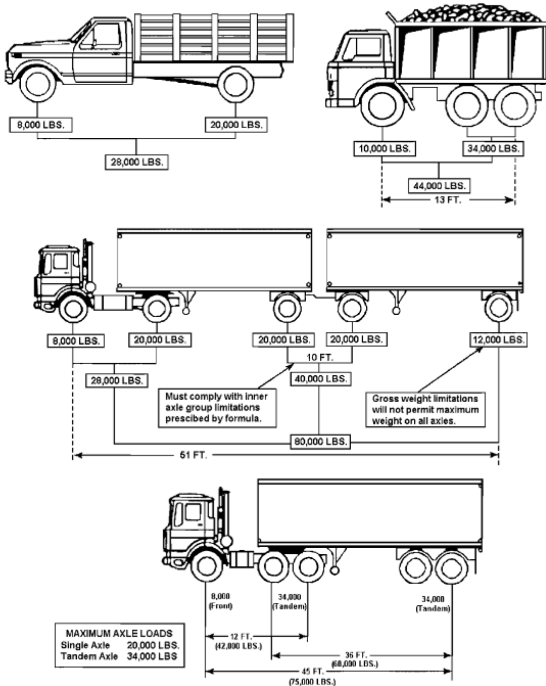
Figure 2-1 Maximum Weights
